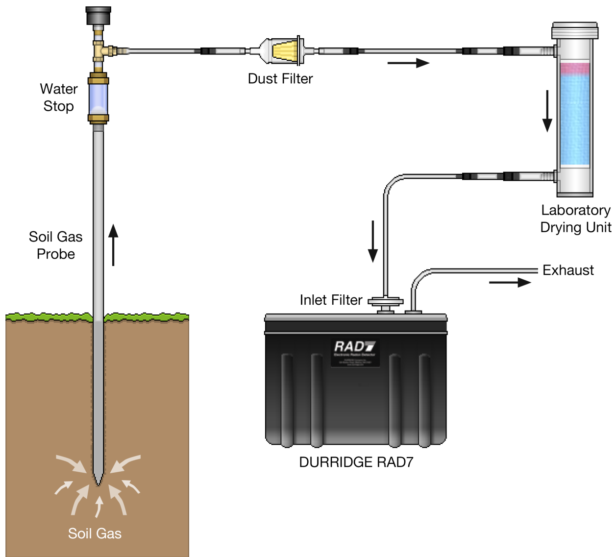
Figure 3 Soil Gas Probe standard configuration
