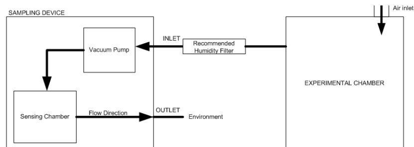
Figure 5: Open Loop
